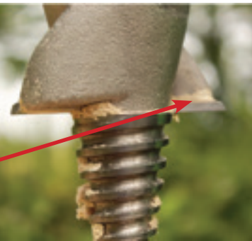
High-quality pilot tip
